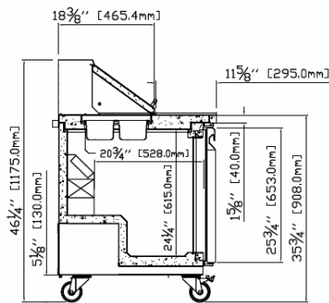
RIGHT VIEW
